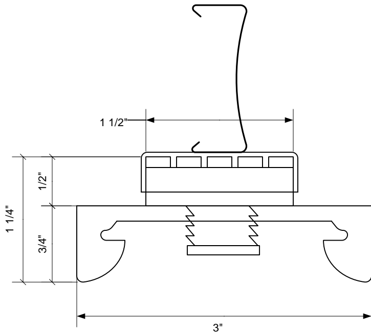
PROFILE VIEW
